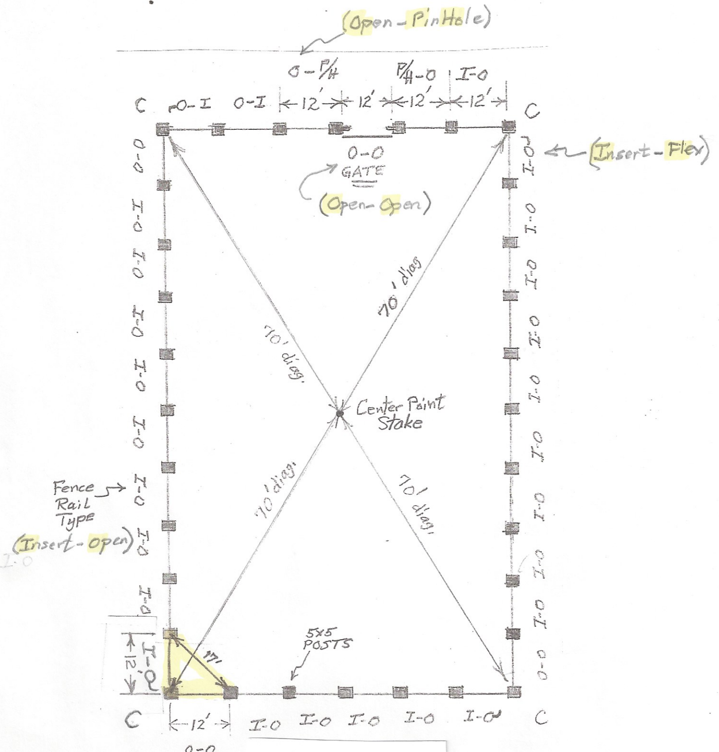
Figure 2 120' x 72' Arena Layout
